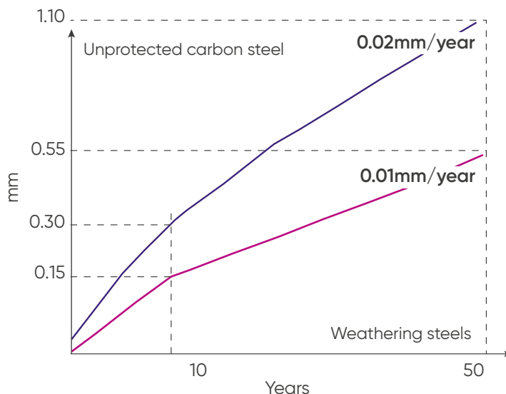
Figure 1: Annual steel loss due to corrosion (in mm) measured in accordance with ISO 12944-2 for a C4 environment.
