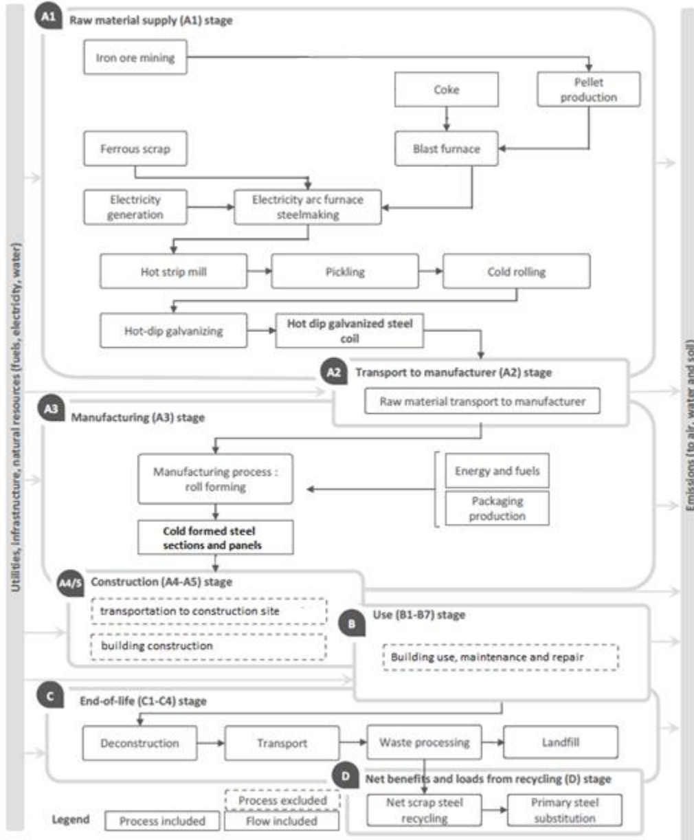
Figure 1: Process flow diagram for steel deck production
