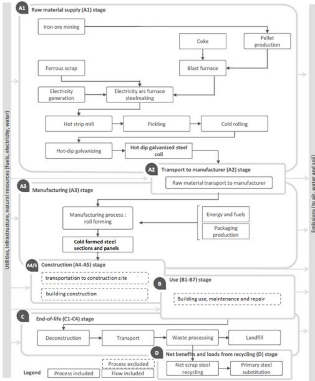
Figure 1: Process flow diagram for cold formed sections
